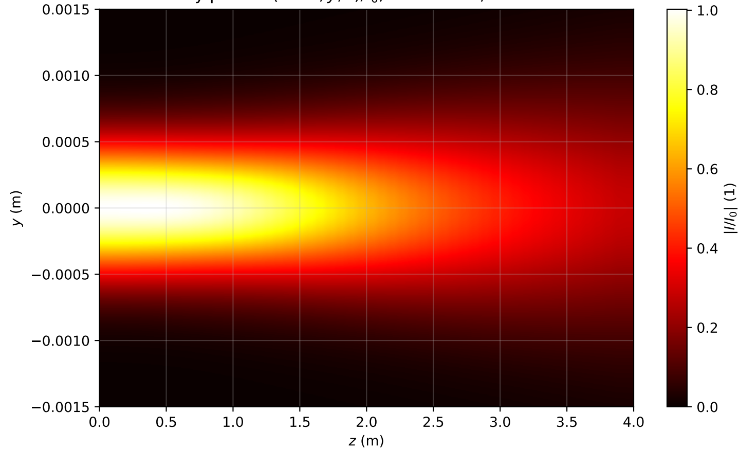
Intensity profile I(x=0, y, z)/I_0 , P_{in}=0.3P_{cr} , artificial time
